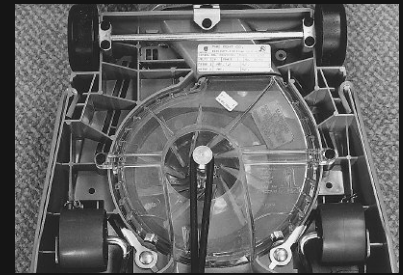
A clear and easy to clean fan cover
